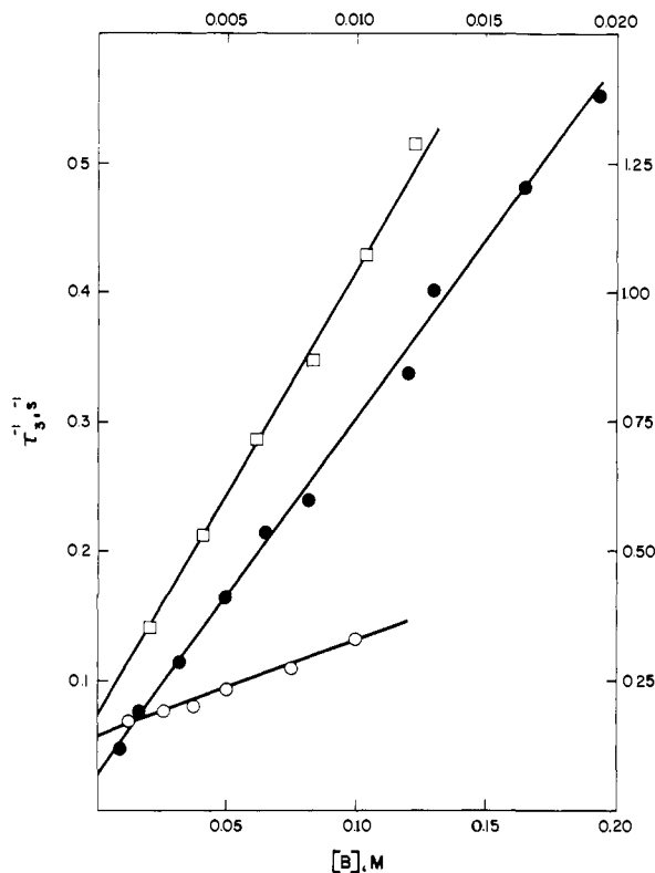
Figure 5. General base catalysis of slow process ( \tau_3^{-1} ) in pH-jump experiments, representative plots. (□) \text{HCOO}^- , pH 5.51 (left and bottom axes); (O) \text{ClCH}_2\text{COO}^- , pH 3.71 (left and bottom axes); (●) 4-picoline, pH 4.14–4.23 (right and top axes).
