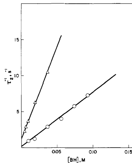
Figure 4. General acid catalysis of fast process ( \tau_2^{-1} ) in pH-jump experiments, representative plots. ( \Delta ) \text{ClCH}_2\text{COOH} , pH 3.76; ( \circ ) \text{AcOH} , pH 4.70.
