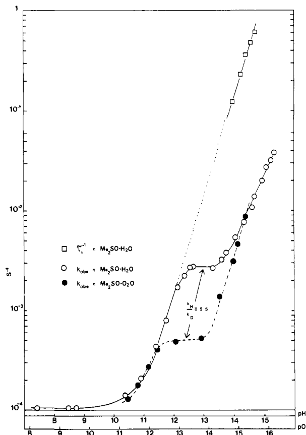
Figure 1. Rate-pH profiles. k obsd refers to overall hydrolysis reaction; τ 1 -1 refers to OH - addition to 2 (eq 1 and 2).
